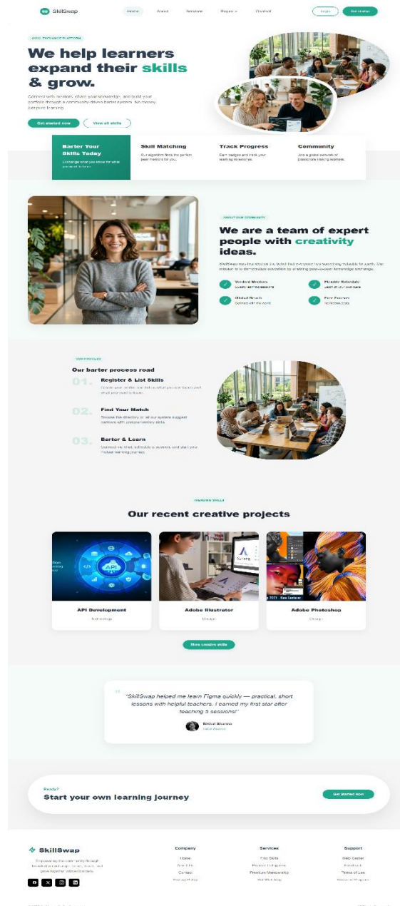
Figure 1: Landing page
